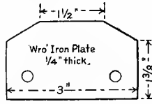
Fig. 4270. STOP-BAR PLATE. To support Stop-bar.
